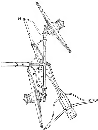
ACKERMAN'S MOVABLE AXLE.
